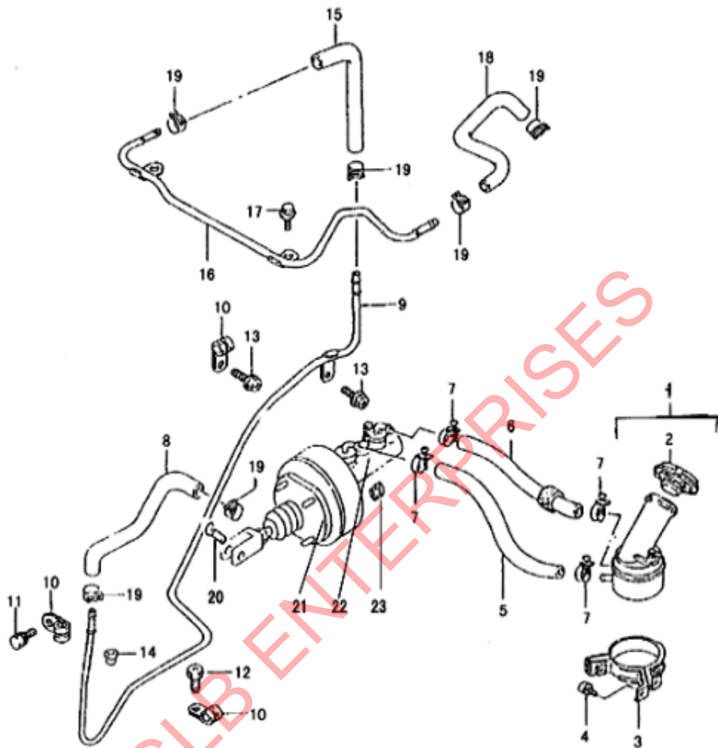
FIGURE 55 BRAKE MASTER CYLINDER AND BOOSTER
