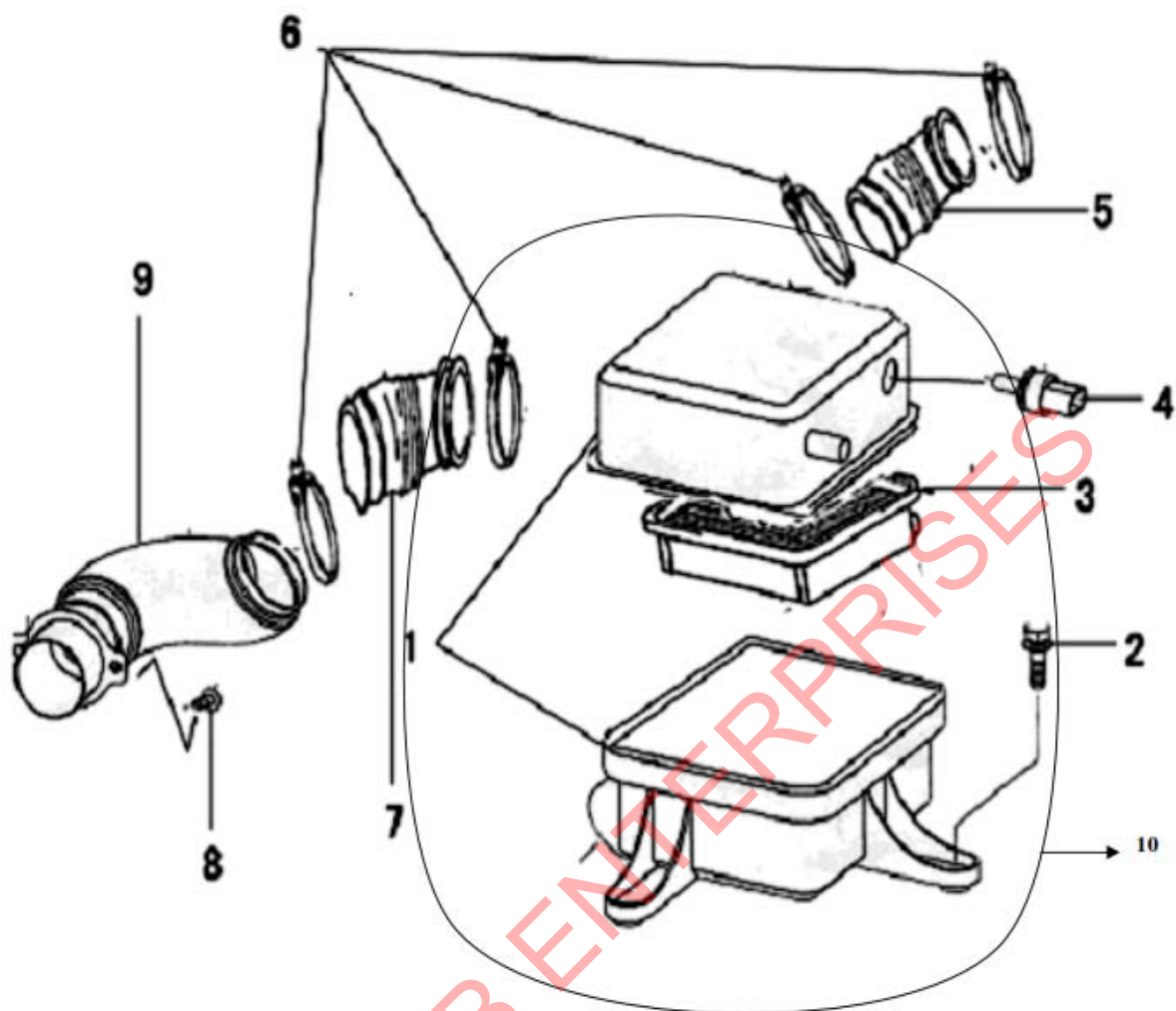
FIGURE 25 AIR FILTER
