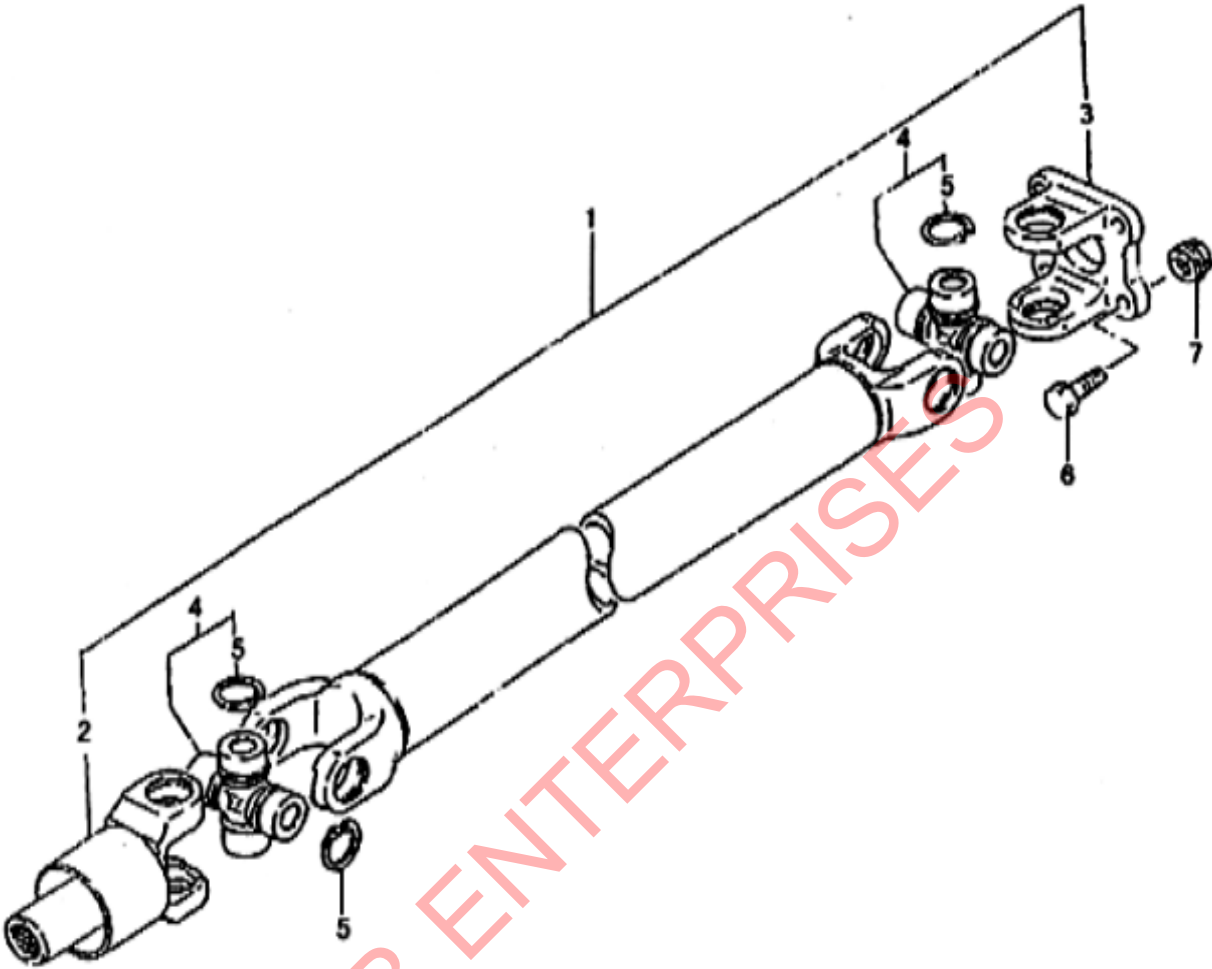
FIGURE 40 DRIVE SHAFT
