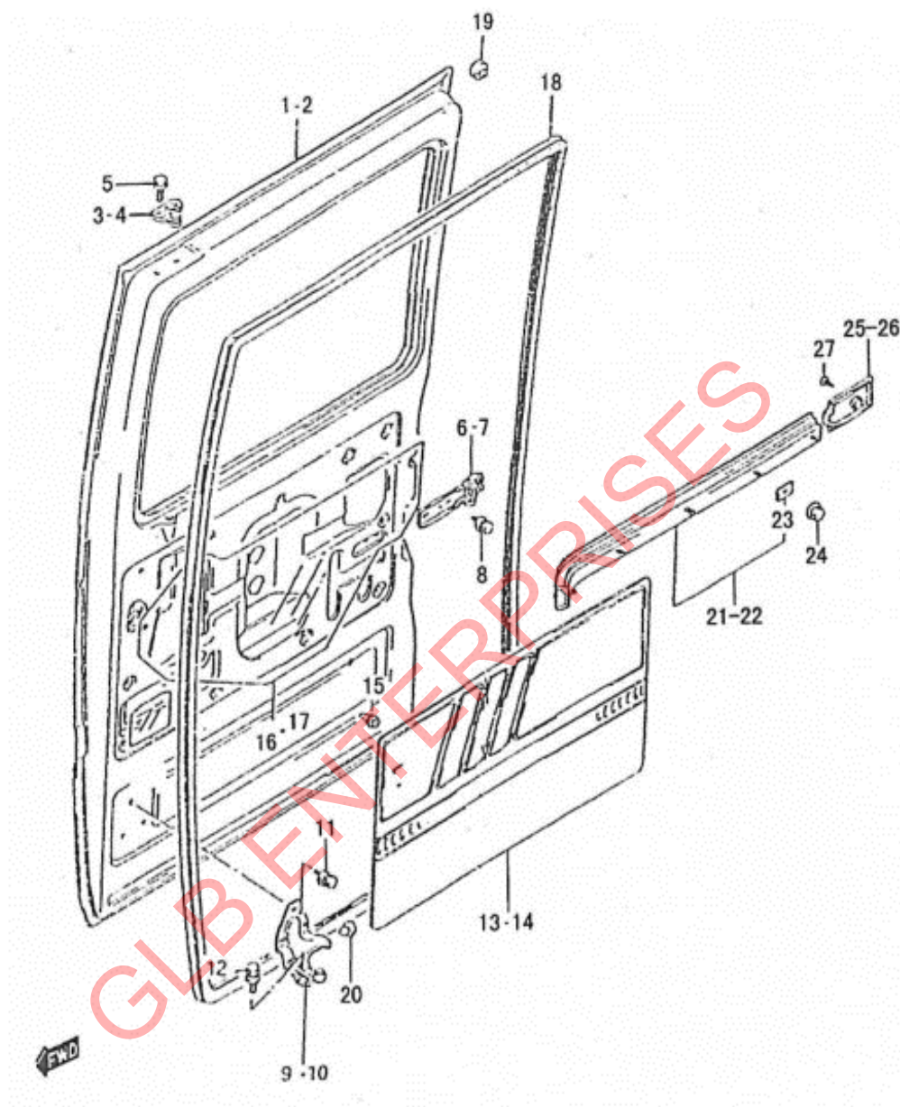
FIGURE 94 SLIDING DOOR
