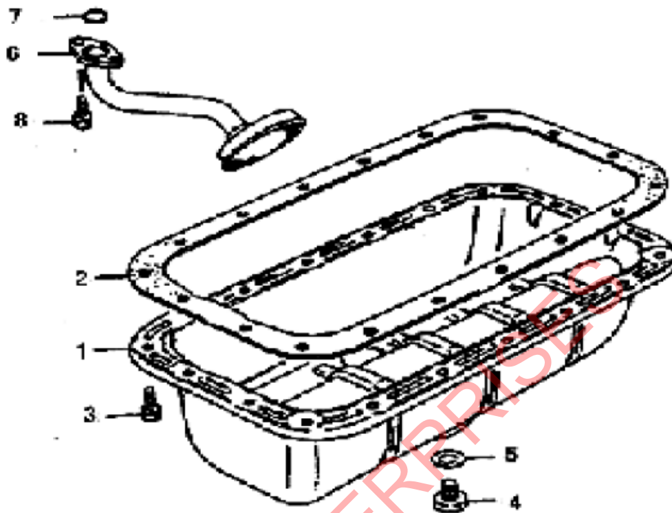
FIGURE 8 OIL PAN
