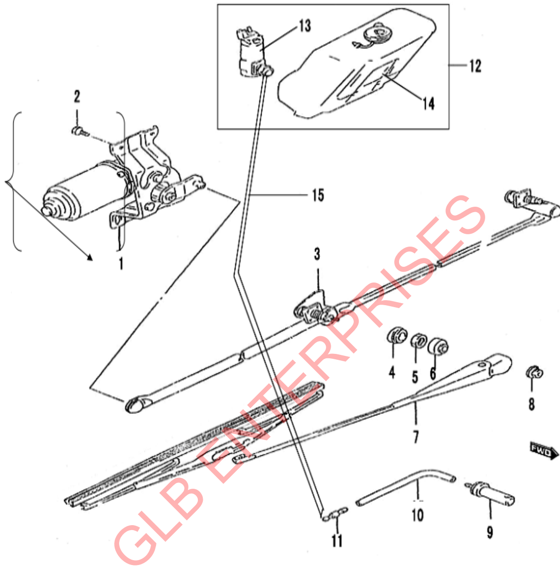
FIGURE 58 WINDSHIELD WIPER
