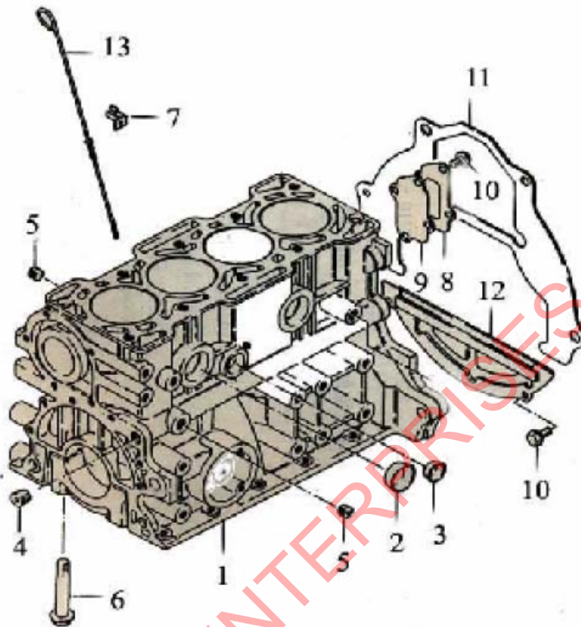
FIGURE 13 CYLINDER BLOCK
