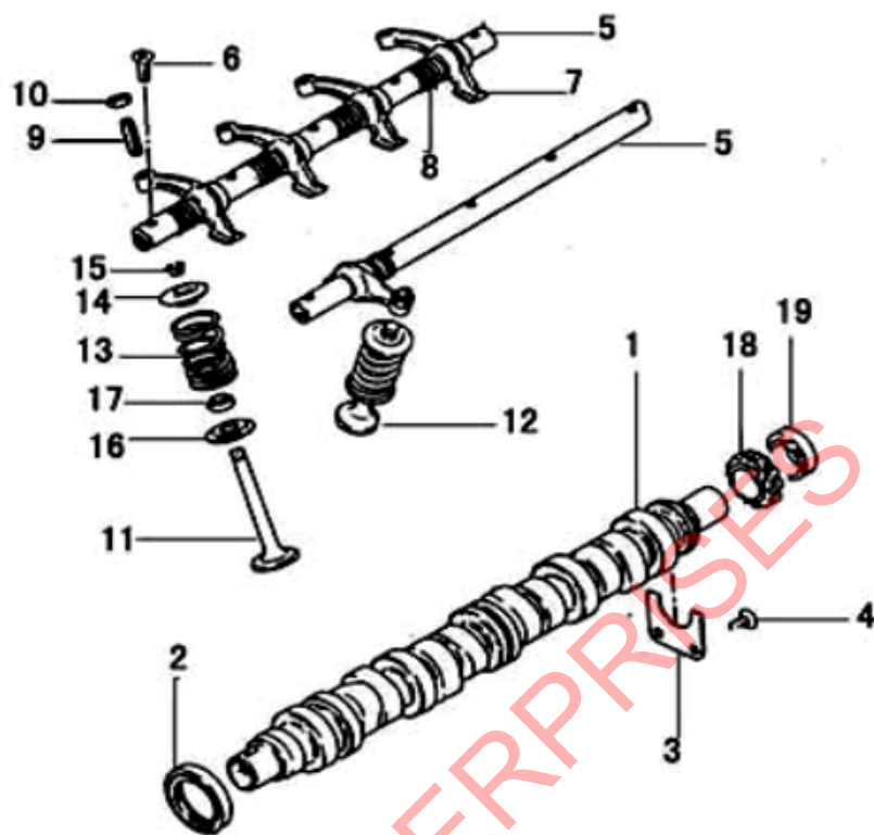
FIGURE 15 CAMSHAFT & VALVE TRAIN
