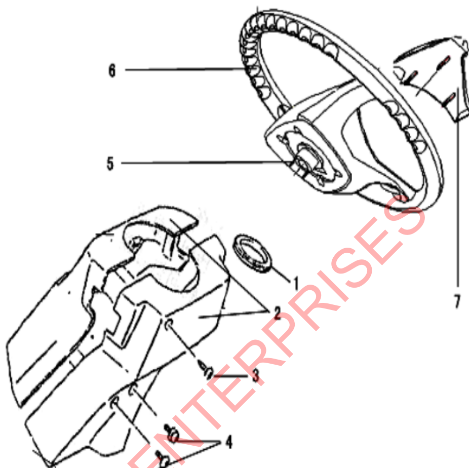
FIGURE 49 STEERING WHEEL
