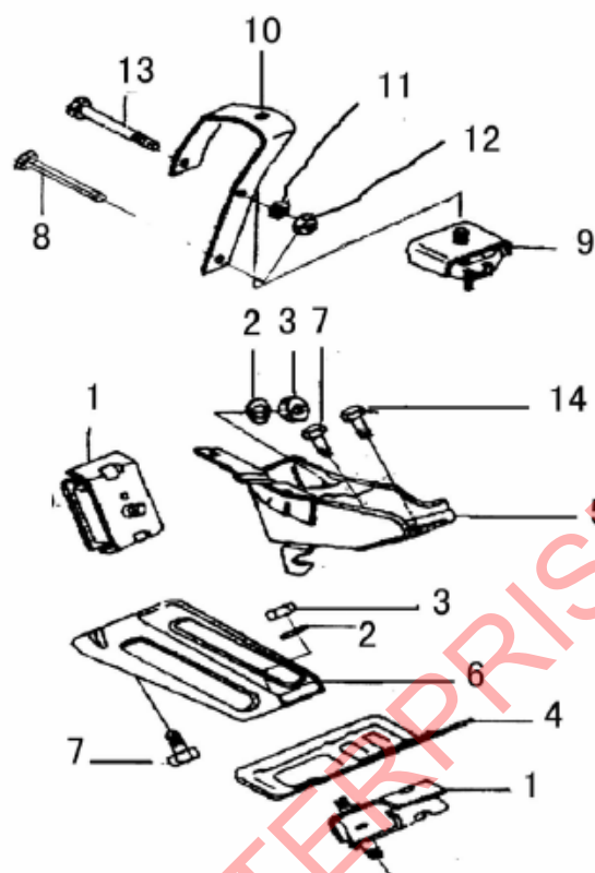
FIGURE 4 REAR MOUNTING CUSHION
