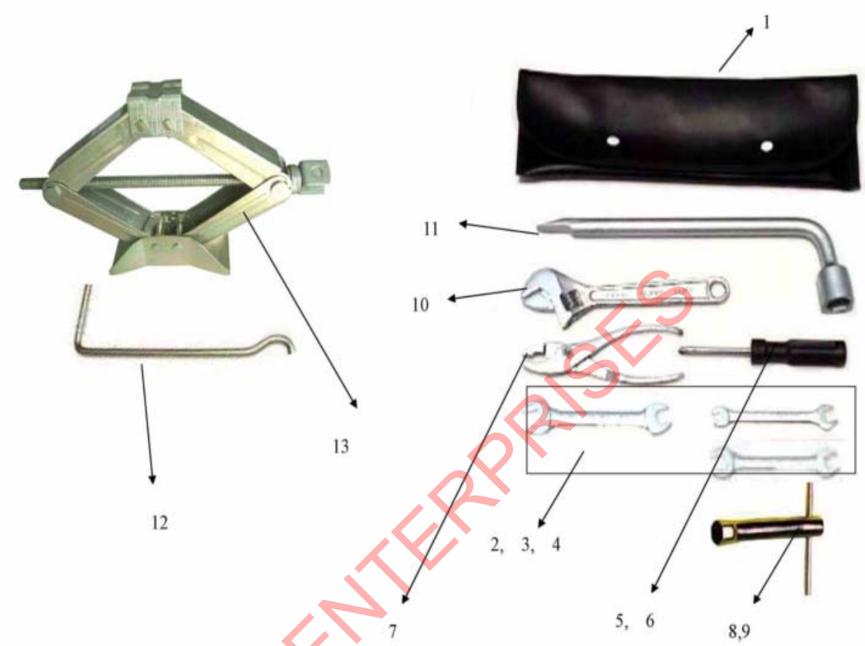
FIGURE 82 TOOL KIT
