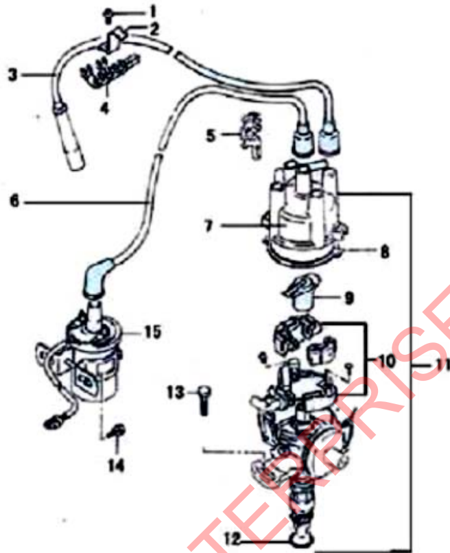
FIGURE 20 DISTRIBUTOR
