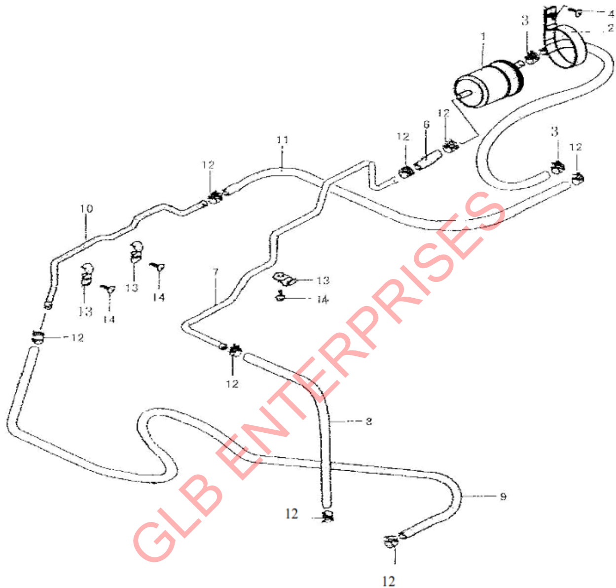
FIGURE 21 FUEL FILTER AND INTERRELATED HOSES EFI
