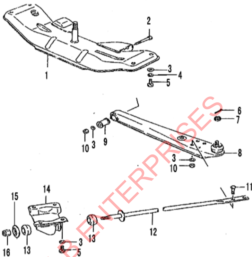
FIGURE 42 FRONT SUSPENSION
