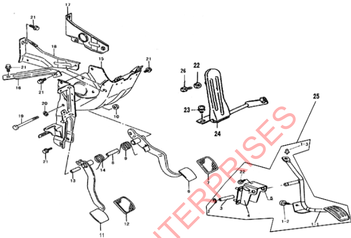
FIGURE 30 BRAKE, CLUTCH & ACCELERATOR PEDAL
