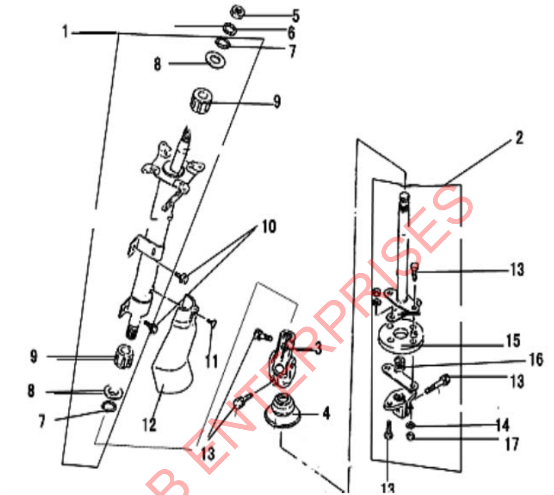
FIGURE 50 STEERING SHAFT
