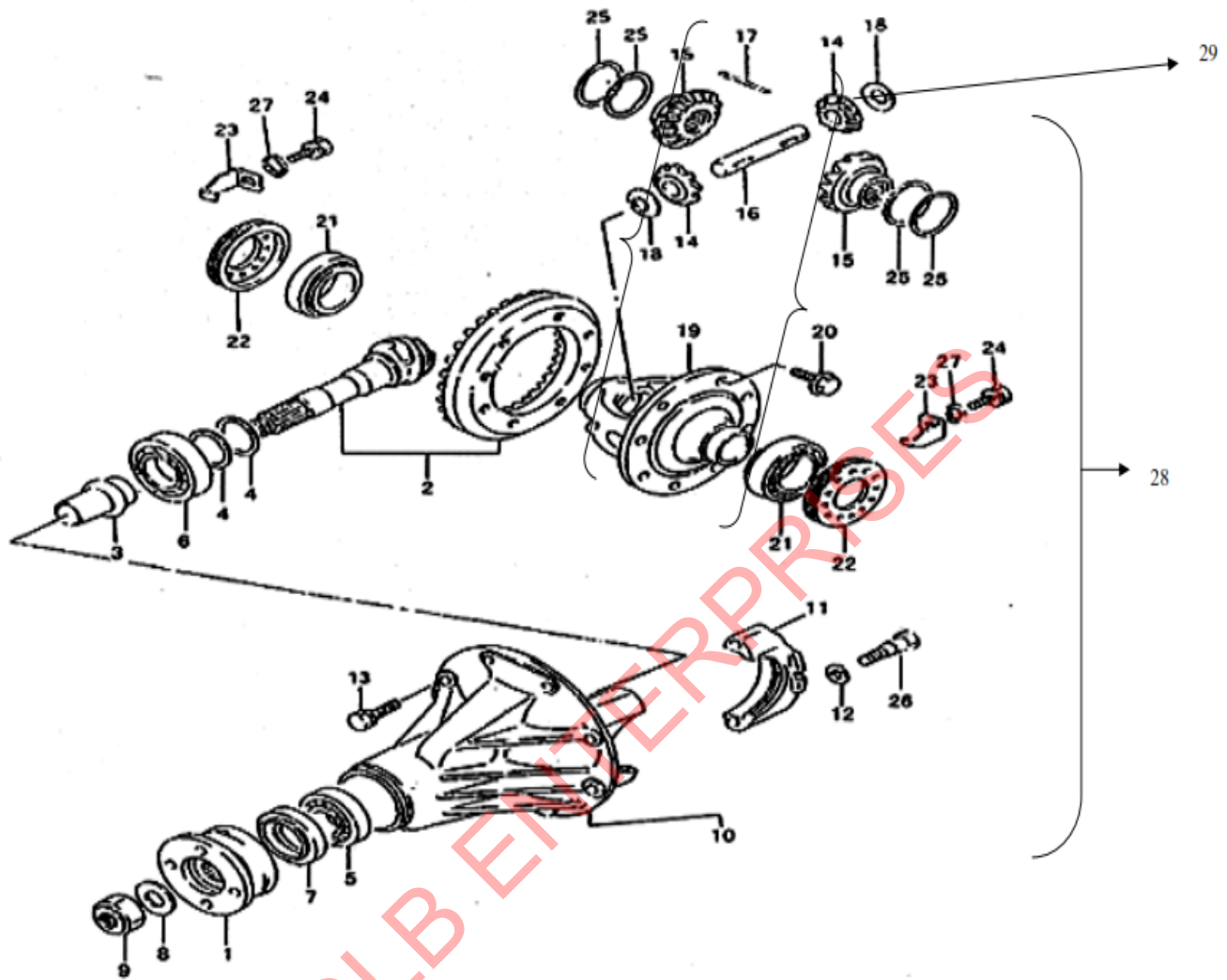
FIGURE 44 REAR END
