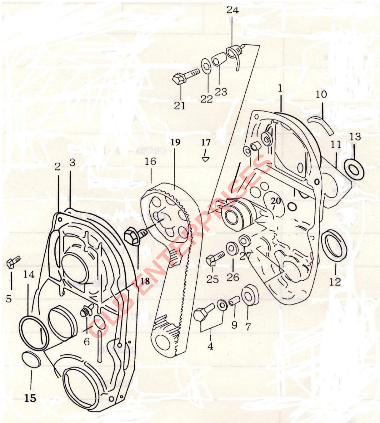
FIGURE 8 TIMING BELT & COVER
