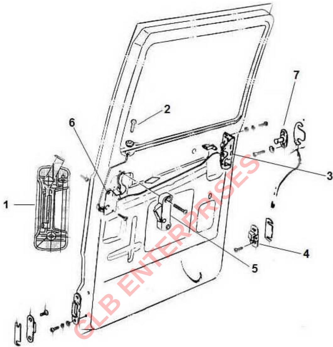
FIGURE 69 SLIDING DOOR LOCKS VAN
