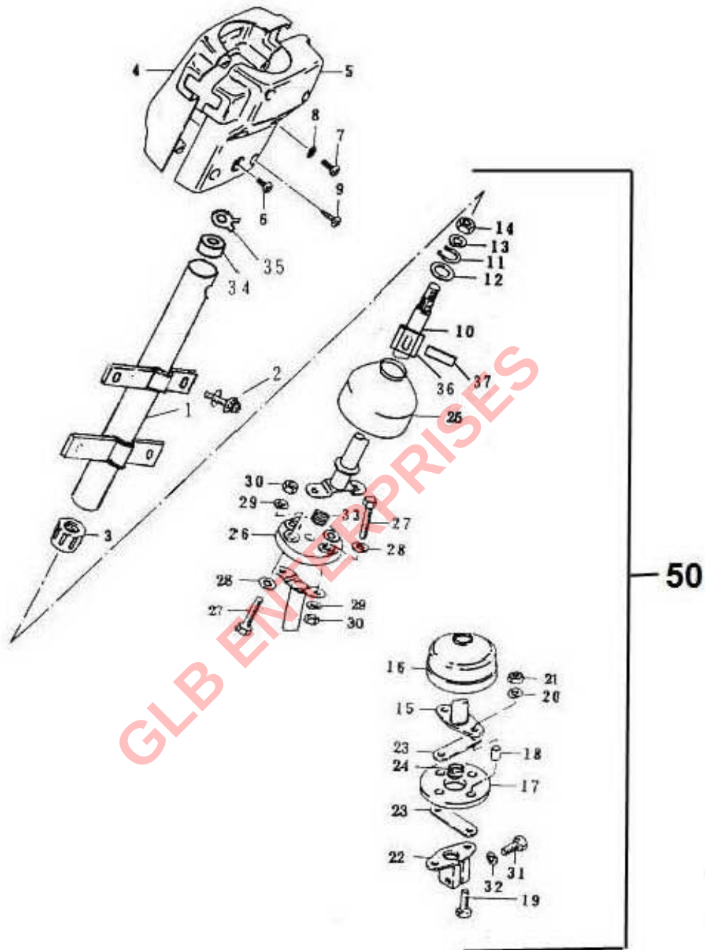
FIGURE 47 STEERING COLUMN
