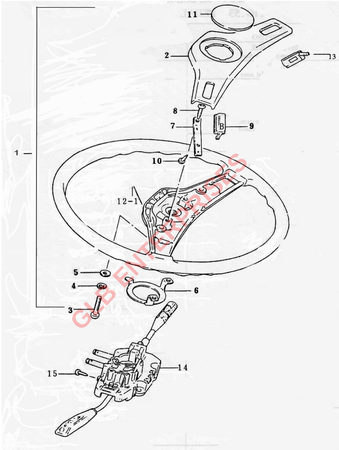
FIGURE 46 STEERING WHEEL
