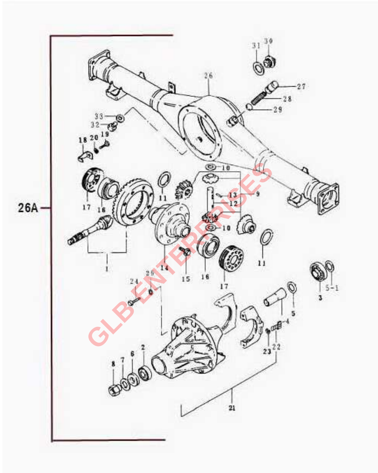
FIGURE 44 REAR END
