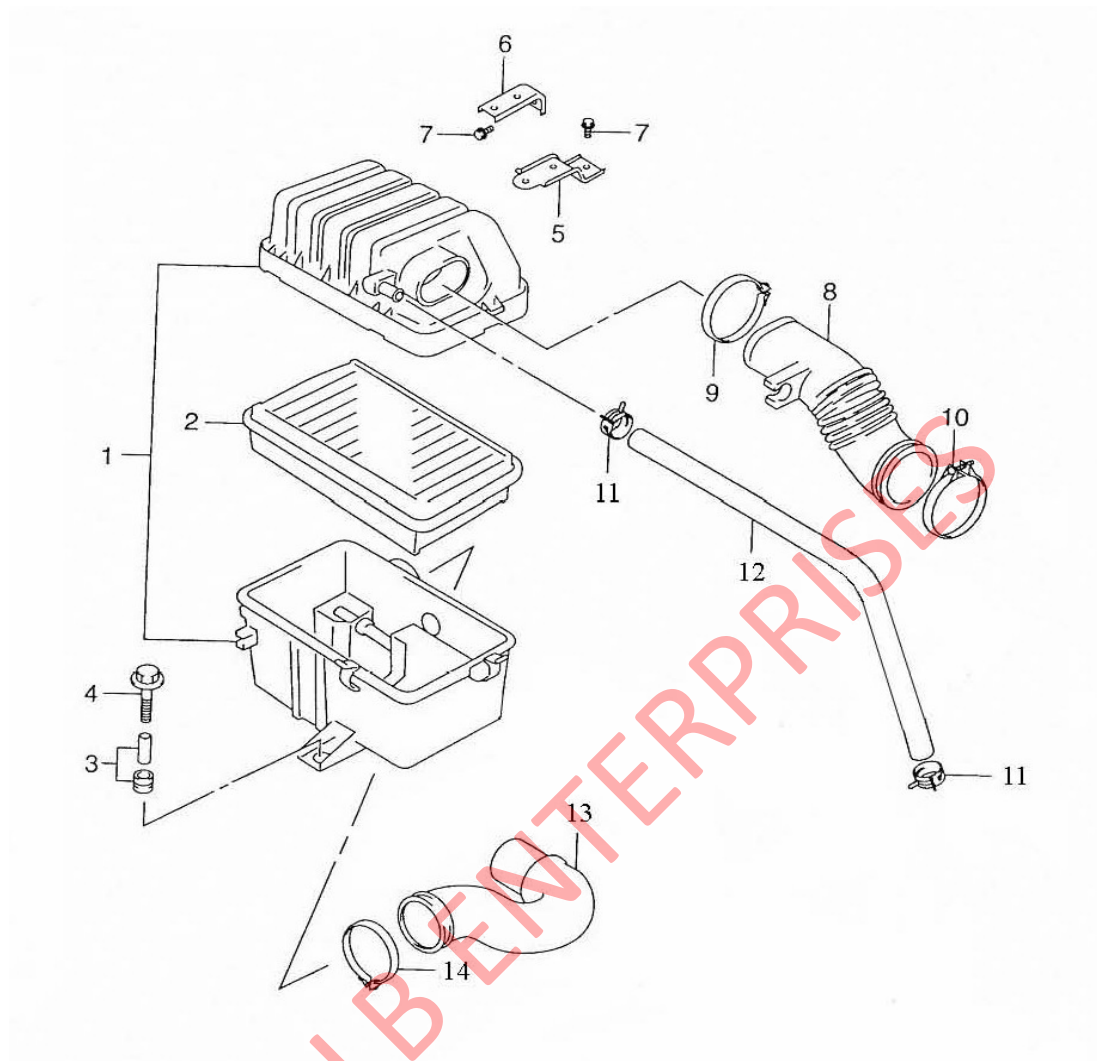
FIGURE 12 AIR CLEANER HOUSING
