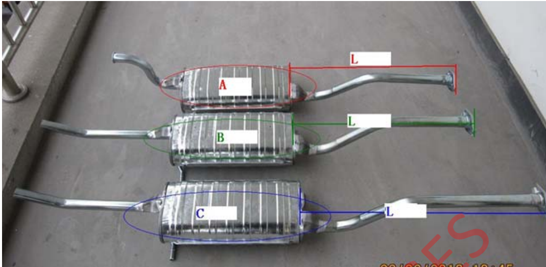
FIGURE 14 MUFFLER
