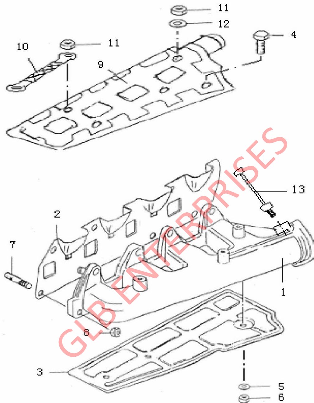
FIGURE 13 EXHAUST MANIFOLD
